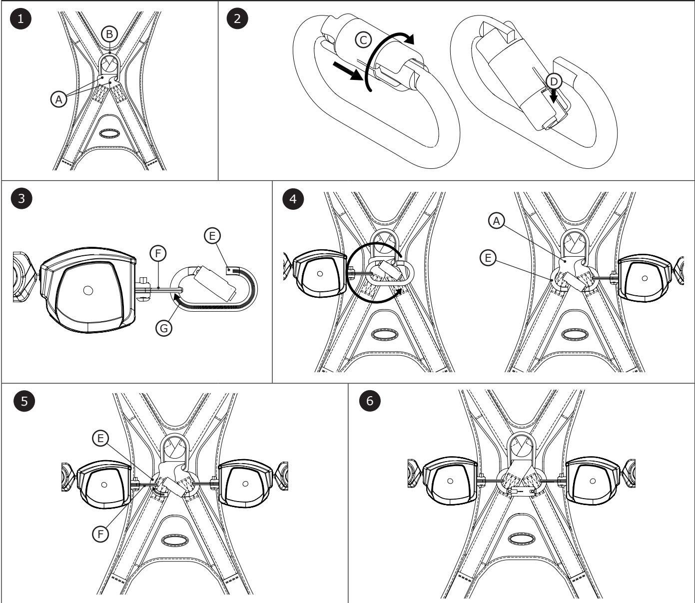
Figure 9 - Carabiner Interface
